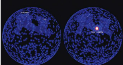
Before and after Fermi LAT views of GRB 130427A, centered on the north galactic pole
